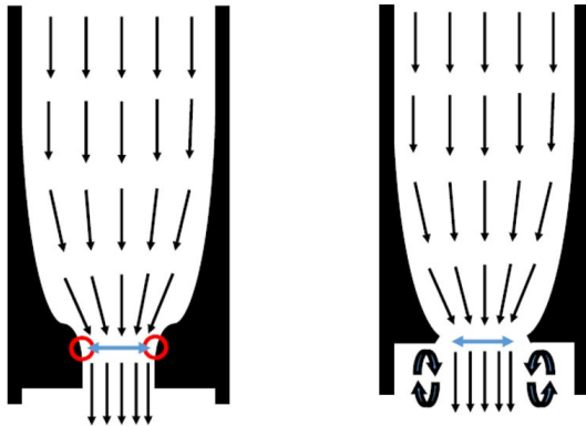
High cavitation risk in insert
