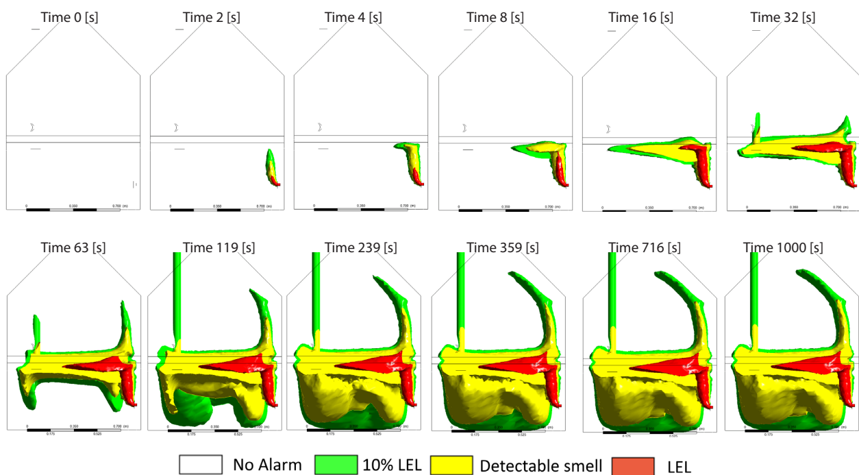
Figure 5 Concentration of natural gas as a function over time
