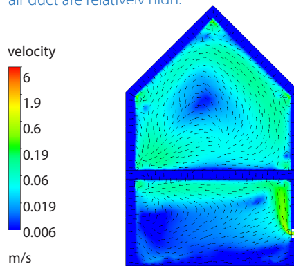
Figure 3 Flow velocity at cross-sectional plane at leakage point
