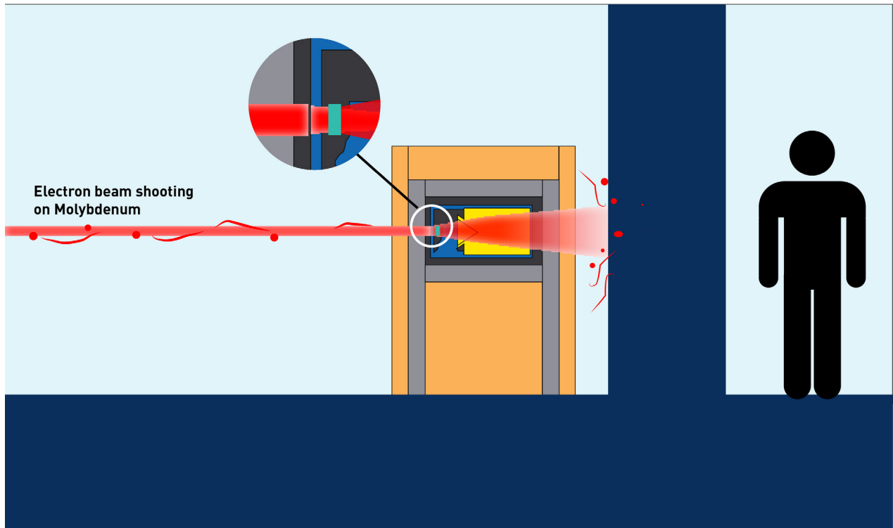
Figure 1: Geometry of the FLUKA model, with the material colors indicated. The beam is incident from the left.
